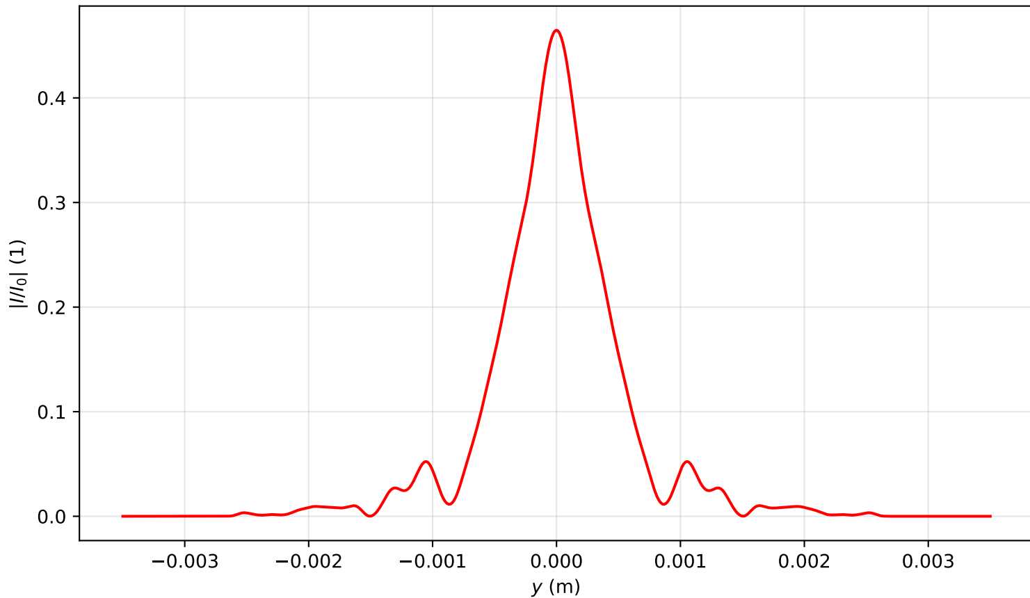
Intensity profile I(x = 0, y, z = 2.149)/I_0 , P_{in}=5.0P_{cr} , artificial time
